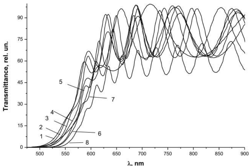
Figura 3. Spectrele de transmisie al straturilor subțiri (As_{45}S_{15}Se_{40})_{1-x}Sn_x x=0 (1), 0.01 (2), 0.02 (3), 0.03 (4), 0.04 (5), 0.05 (6), 0.07 (7), 0.10 (8)
