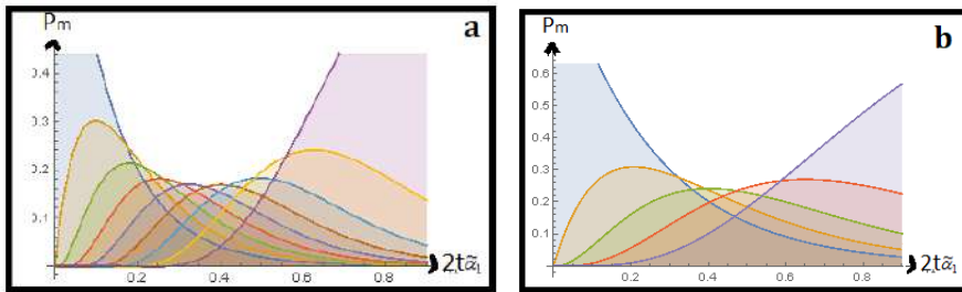
Figure 4. The time dependence of probabilities P_m(t) for the following values of the relative parameters \alpha_2/\alpha_1 = 0.0075 and the number of photons 2j = 8 and 2j = 4
