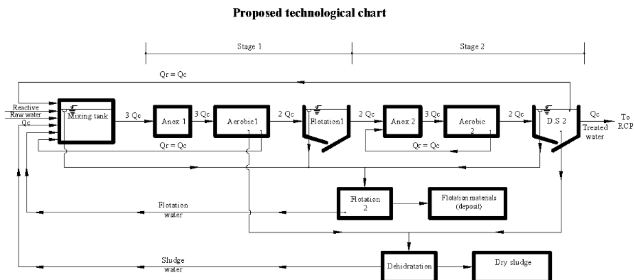
Chart 1 – Technological chart for the industrial wastewater depollution treatment
