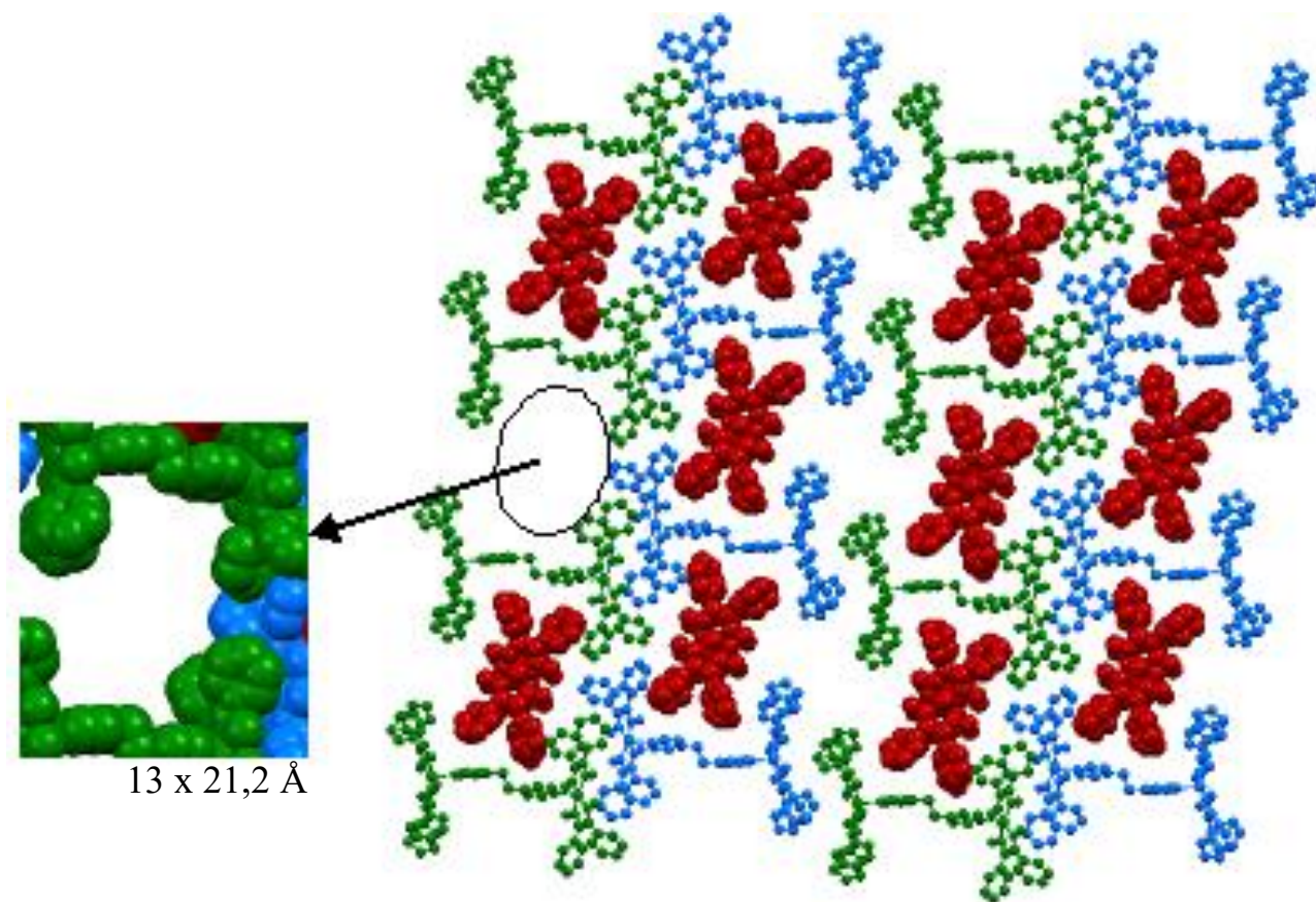
Fig. 5. Formation of intermolecular cavities in [Cu 2 (NioxH) 4 bpe]
